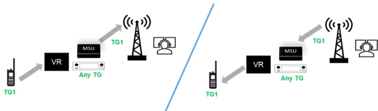
Figure 13: Talkgroup Proxying - Successful PSU Communication
