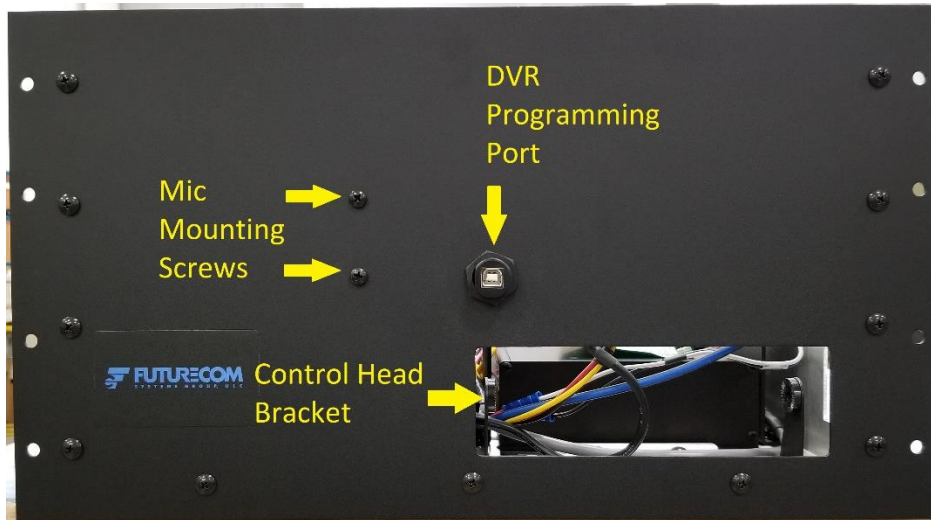
Figure 2 - Rackmount DVRS - As Received (front view)
