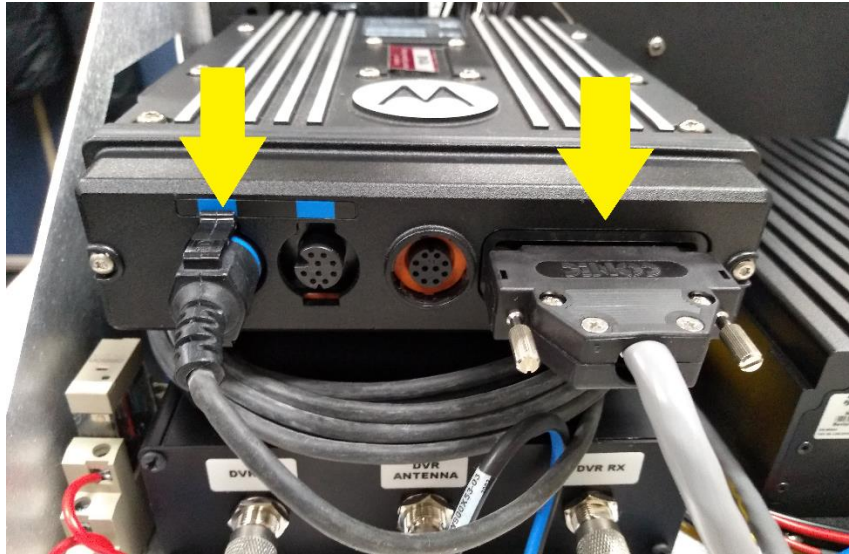
Figure 11 - Installation of the MSU
