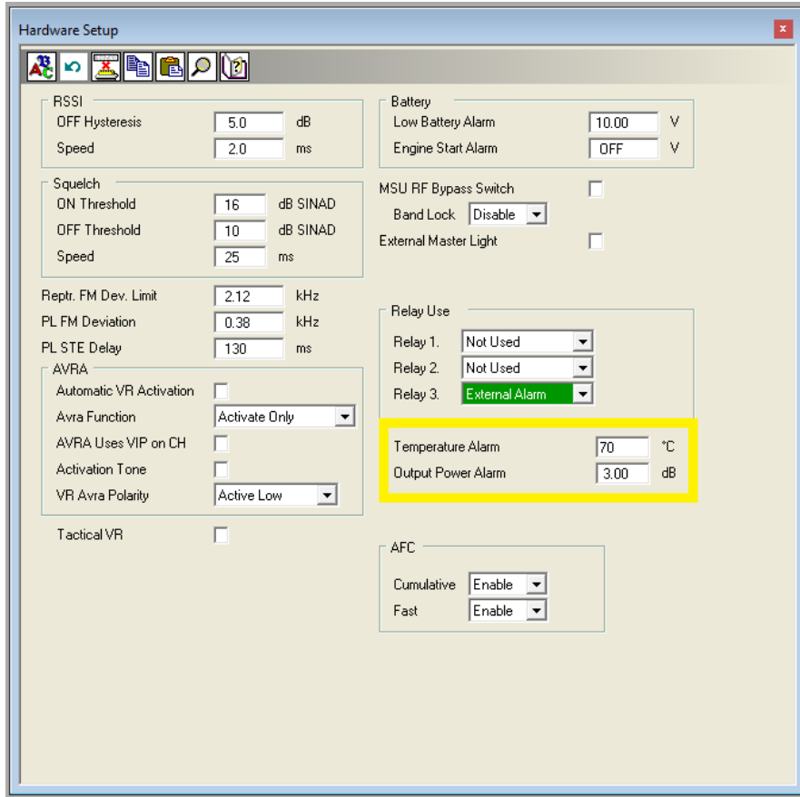
Figure 18 - Alarm threshold values
